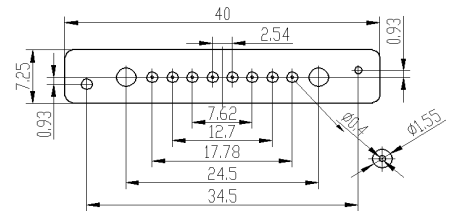
PCB Foot-Print Layout
