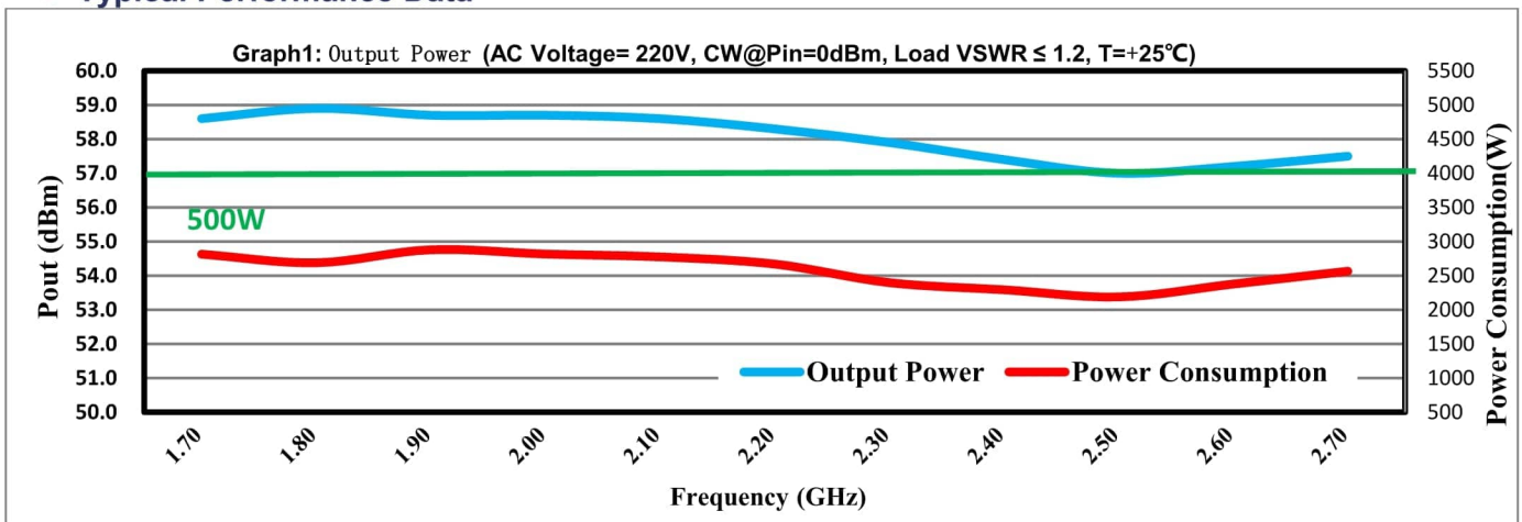
Psat & Power Consumption (CW, Load VSWR≤1.2, 25°C)
