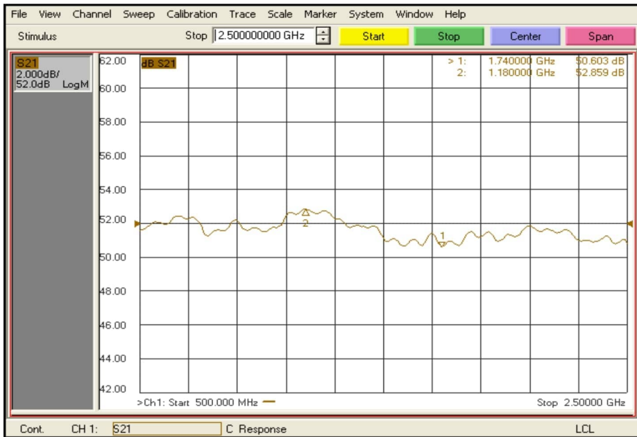
Gain S21 (Pin= 0 dBm, CW, Load VSWR≤1.2, 25°C), Power gain Flatness for reference only
