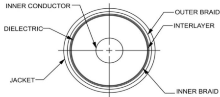
Cable Cross Section
