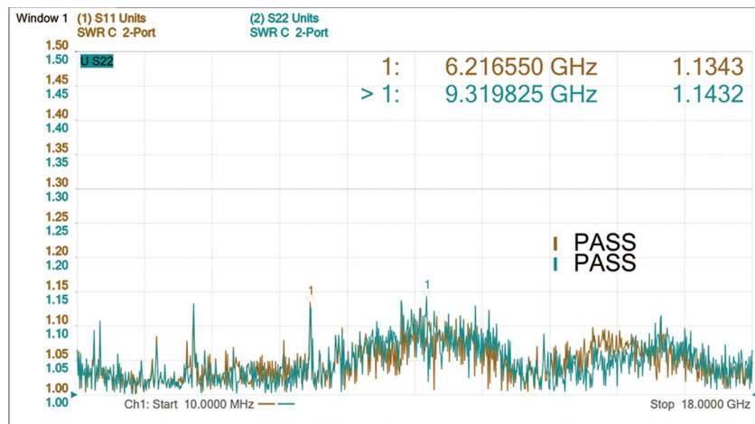
Tested VSWR for A20-07-07-3M/VA2
